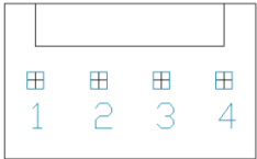
Figure 7: Communication/Power Header
