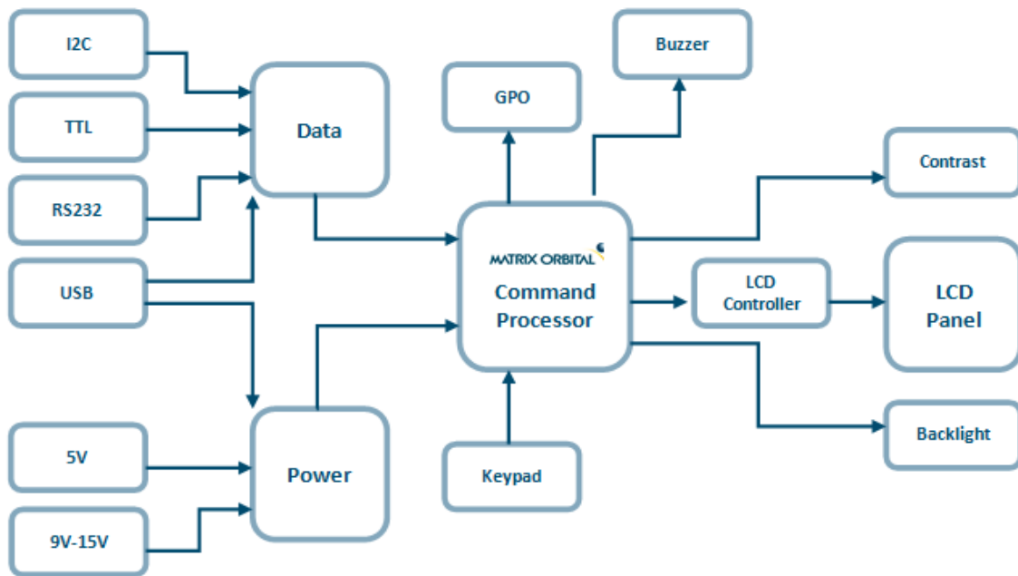
Figure 15: Functional Diagram
